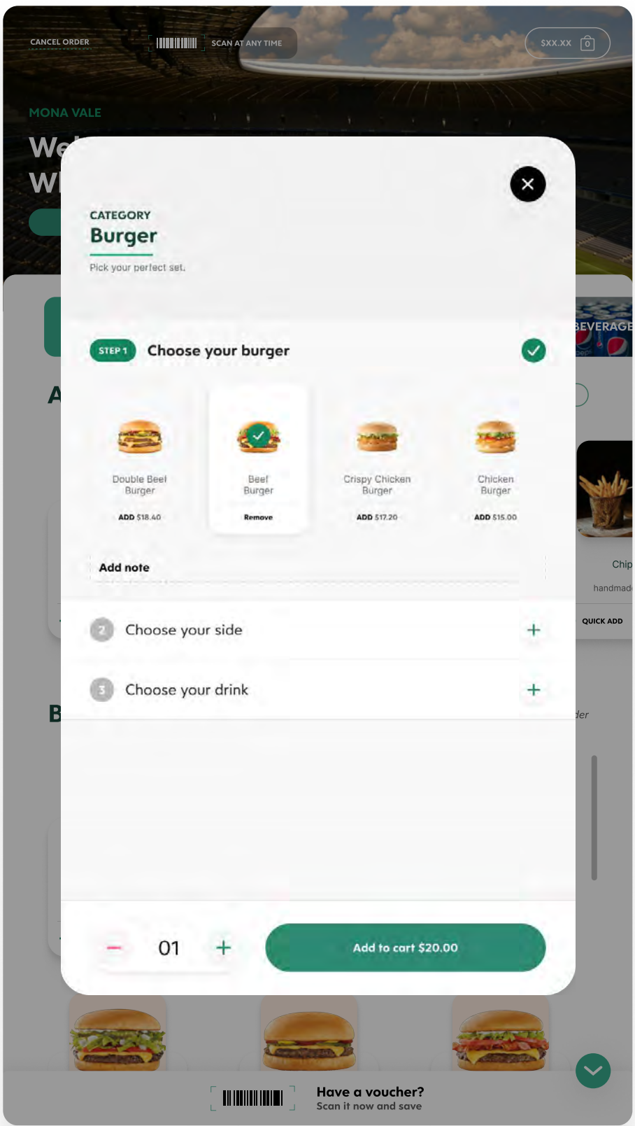
Menu flow
